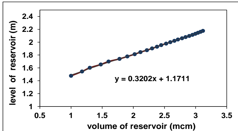
Figure 2. Line and equation of Maroon dam reservoir type definition.
