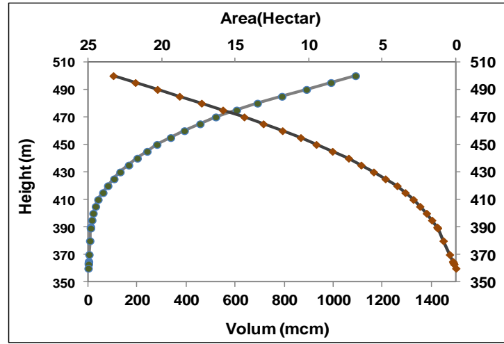
Figure 1. Primary area-volume-height curves of Maroon dam.
